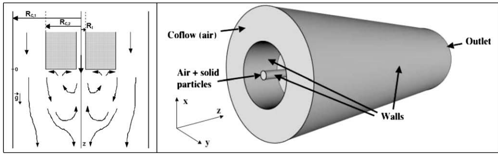
Fig. 1. Configuration of Borée et al. [1]. The dimensions are: R_l = 0.010 m, R_{c1} = 0.075 m, R_{c2} = 0.150 m. The ducts and the chamber are respectively 2 m and 1.5 m long.
