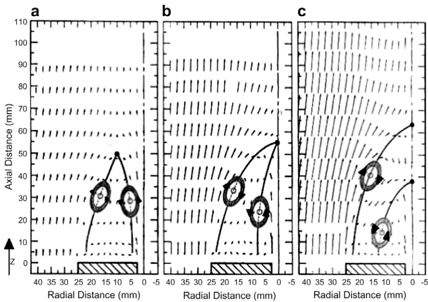
Fig. 2. Plots of the measured mean velocity vectors in a bluff body stabilised methane jet for \bar{U}_{f,1}/\bar{U}_{f,c} = 2.8 (a), \bar{U}_{f,1}/\bar{U}_{f,c} = 1.4 (b), and \bar{U}_{f,1}/\bar{U}_{f,c} = 0.84 (c). Black dots show the location of the stagnation points and round arrays give the direction of rotation of the shear layer vortices. From Schefer et al. [17].
